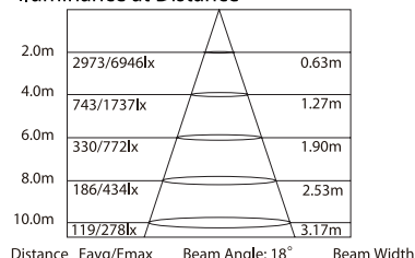
Illuminance at Distance
